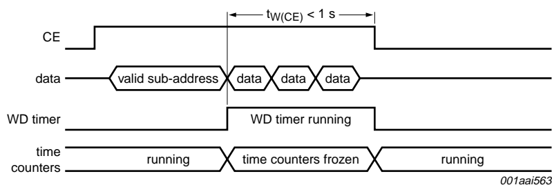
a. Correct data transfer: read or write
