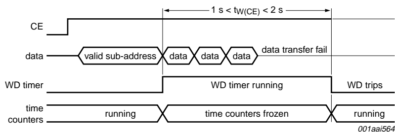
b. Incorrect data transfer; read or write
