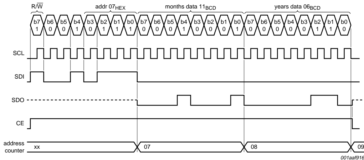
Fig 25. Serial bus read example
