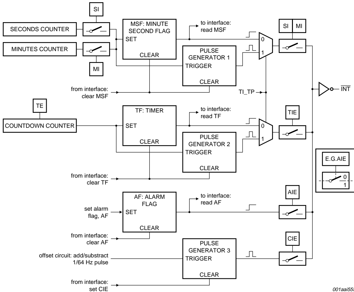
Fig 16. Interrupt scheme
