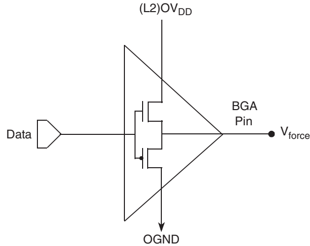
Figure 34. Alternate Driver Impedance Measurement Circuit
