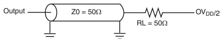
Figure 10. AC Test Load for the 60x Interface
