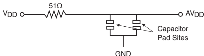
Figure 31. PLL Power Supply Filter Circuit No.2
