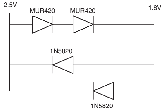
Figure 32. Example Voltage Sequencing Circuits
