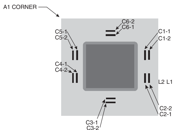
Figure 26. Substrate Bypass Capacitors for the PC7410
