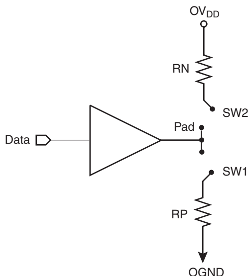
Figure 33. Driver Impedance Measurement Circuit
