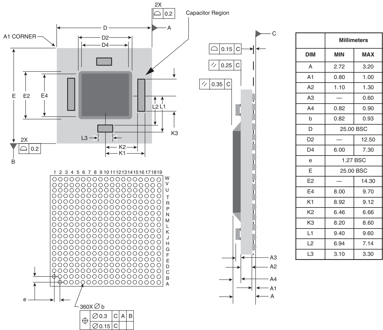
Figure 25. Mechanical Dimensions and Bottom Surface Nomenclature of the 360-ball CBGA Package
