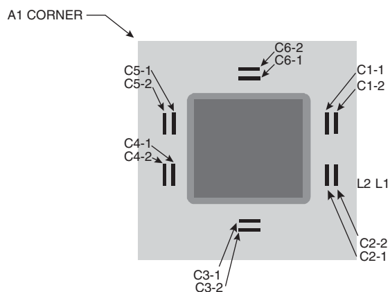
Figure 28. Substrate Bypass Capacitors for the PC7410
