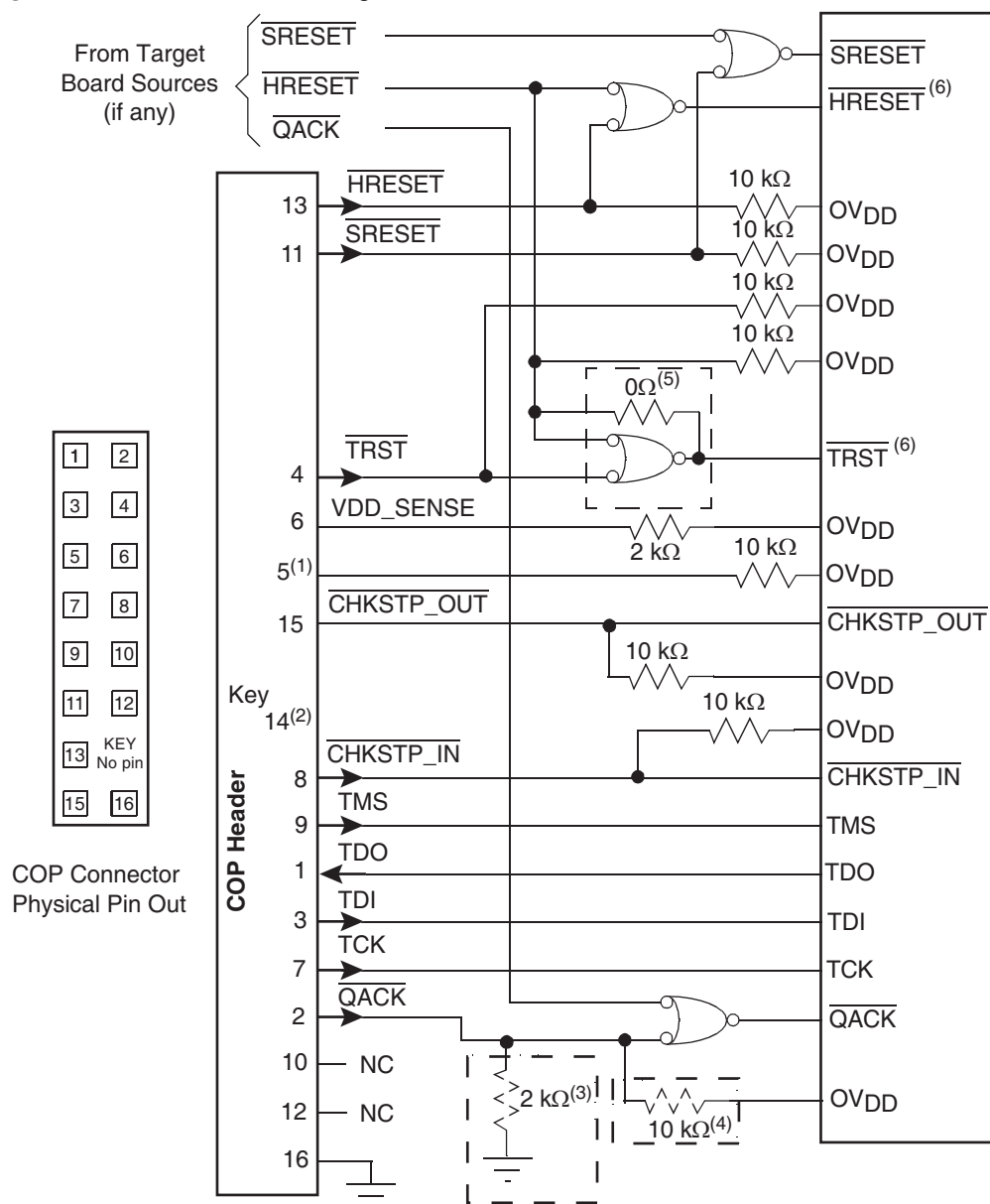
Figure 35. COP Connector Diagram
