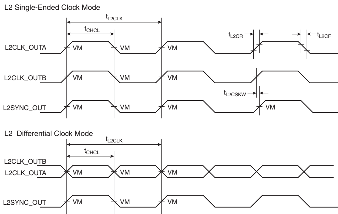
Figure 12. L2CLK_OUT Output Timing Diagram
