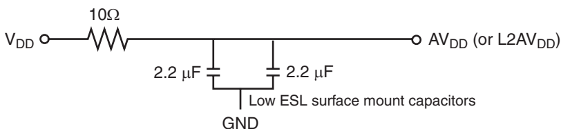
Figure 31. PLL Power Supply Filter Circuit No.2
