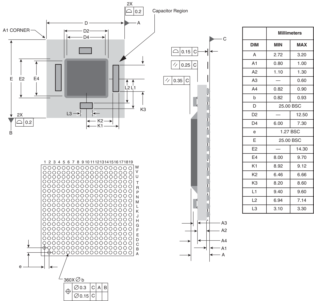
Figure 27. Mechanical Dimensions and Bottom Surface Nomenclature of the 360-ball HiTCE Package
