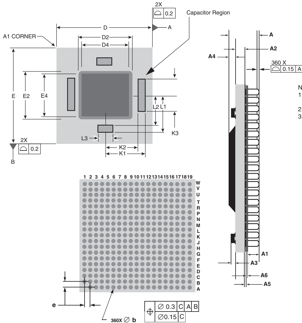
Figure 29. Mechanical Dimensions and Bottom Surface Nomenclature of the 360-column CI-CGA Package
