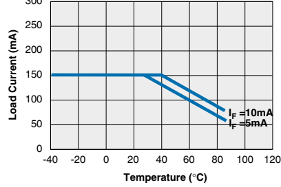
PAA190 Typical Load Current vs. Temperature
