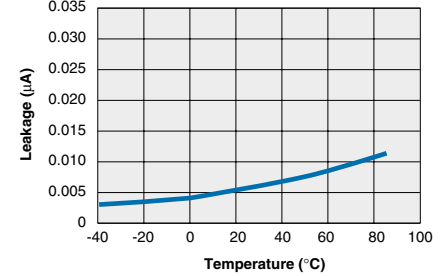
PAA190 Typical Leakage vs. Temperature (Measured across Pins 4 & 6)
