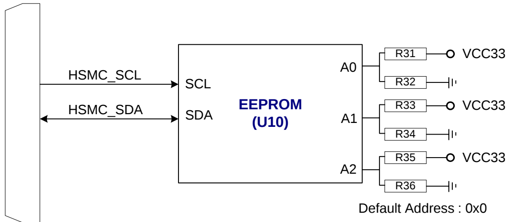
Figure 3.13 The block diagram of the EEPROM and HSMC connector
