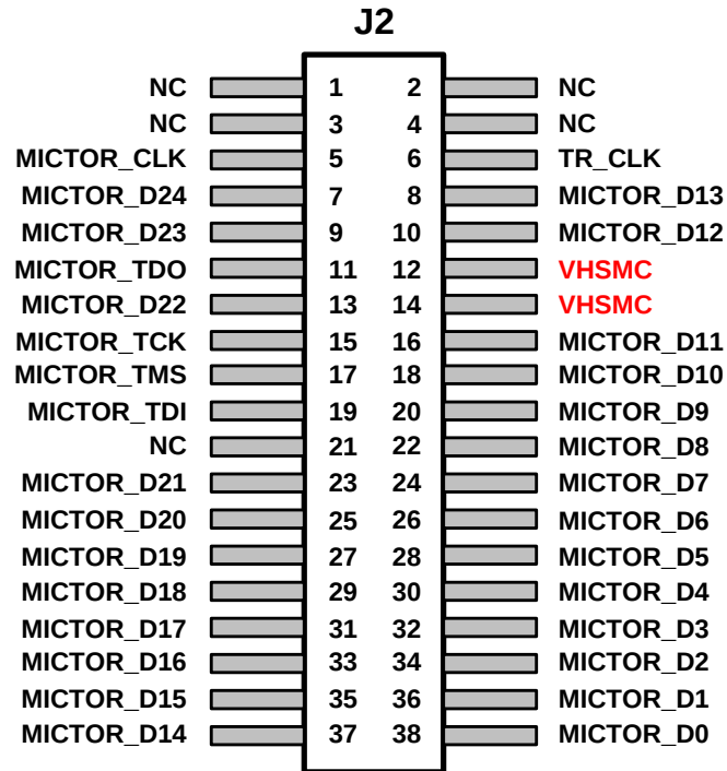
Figure 3.9 Mictor connector pin-outs
