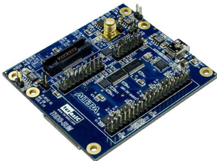
Figure 1.1. The THDB-SUM board
