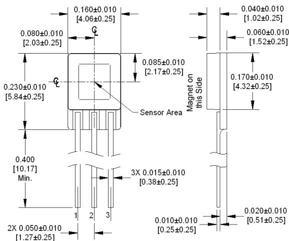
Through Hole
