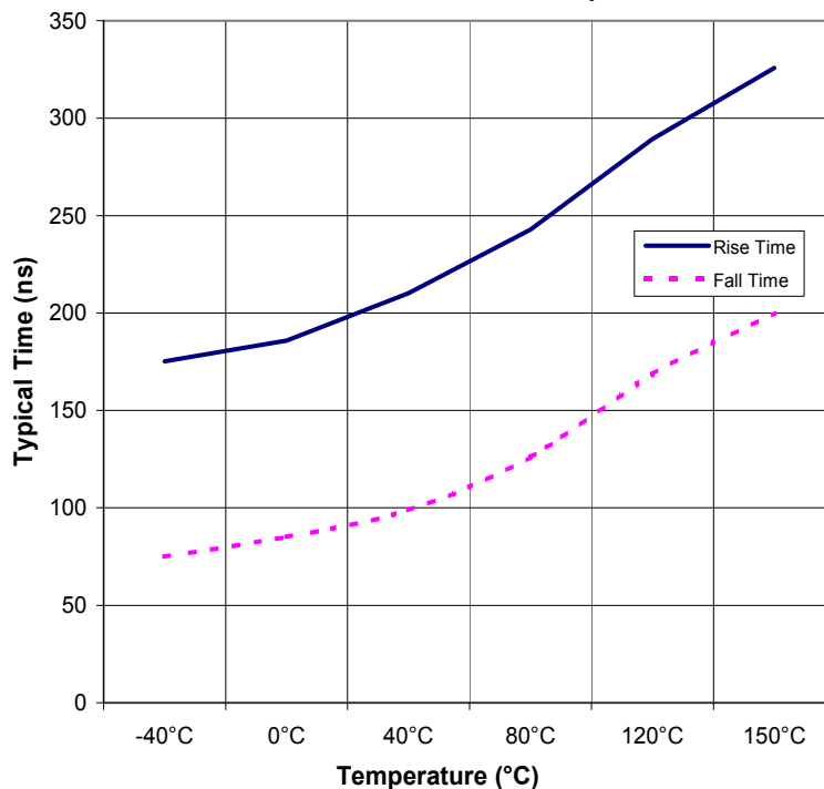
Rise and Fall Time vs Temperature
