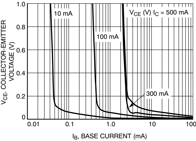
Figure 7. Saturation Region
