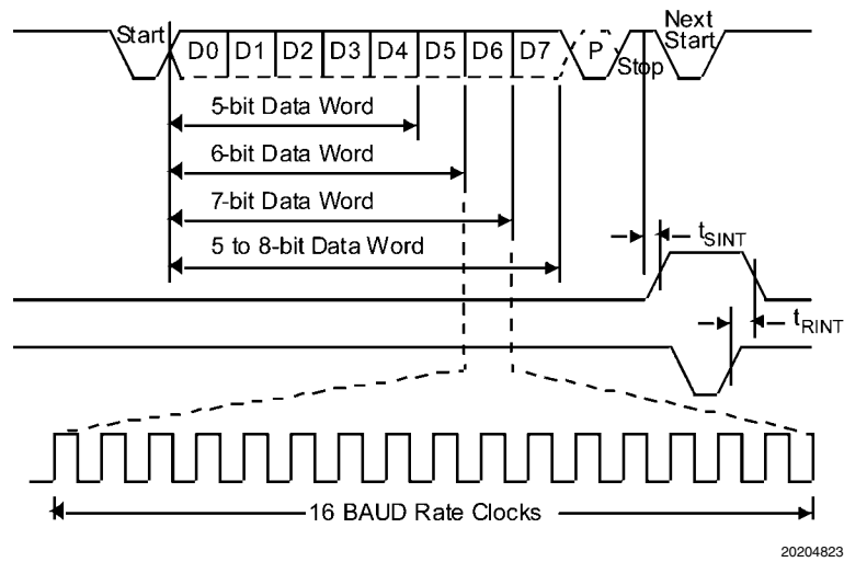
FIGURE 21. Receiver Timing
