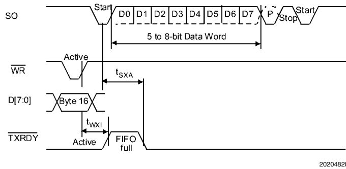
FIGURE 26. Transmitter Timing FIFO Mode
