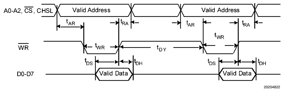
FIGURE 20. Host Interface Write Timing
