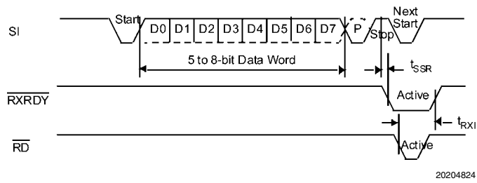
FIGURE 22. Receiver Timing Non-FIFO Mode
