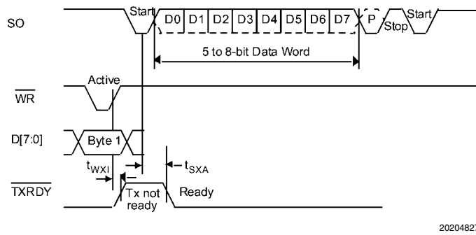
FIGURE 25. Transmitter Timing Non-FIFO Mode
