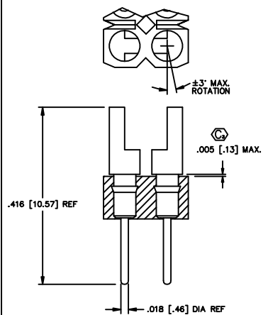
FIG. 8 TERMINAL STYLE -C T-1R2-X
