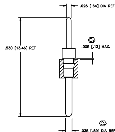
FIG. 4 TERMINAL STYLE -A-2 T-1R7-2-X
