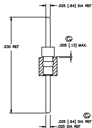
FIG. 3 TERMINAL STYLE -A-1 T-1R7-1-X
