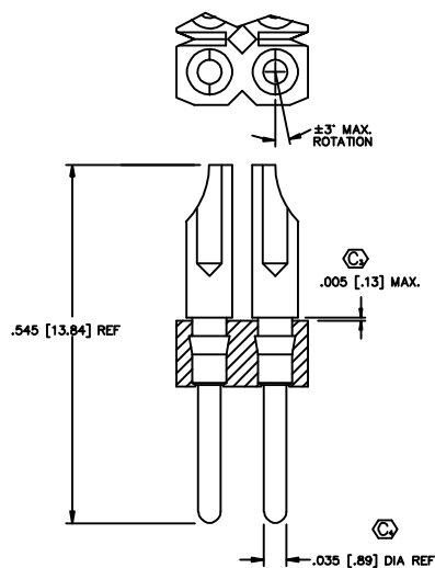
FIG. 7 TERMINAL STYLE -B-2 T-1R8-2-X
