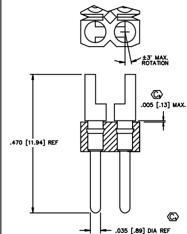
FIG. 10 TERMINAL STYLE -C-2 T-1R9-2-X
