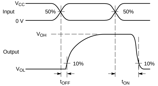
Figure 3. t_{\text{ON}}/t_{\text{OFF}}
