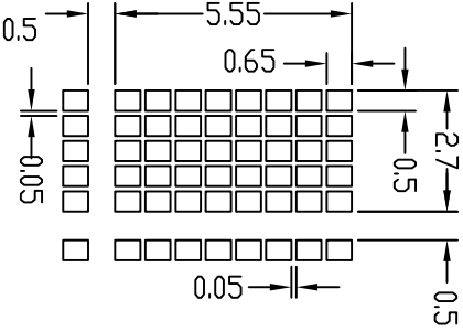
DOTS DETAIL
