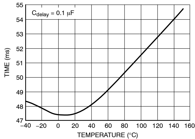
Figure 6. Delay Time
