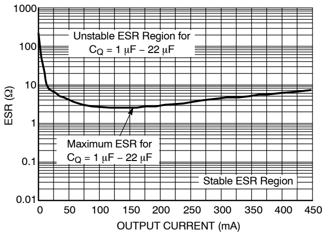
Figure 5. Output Stability with Output Capacitor ESR, 5.0 V and Adjustable Regulator
