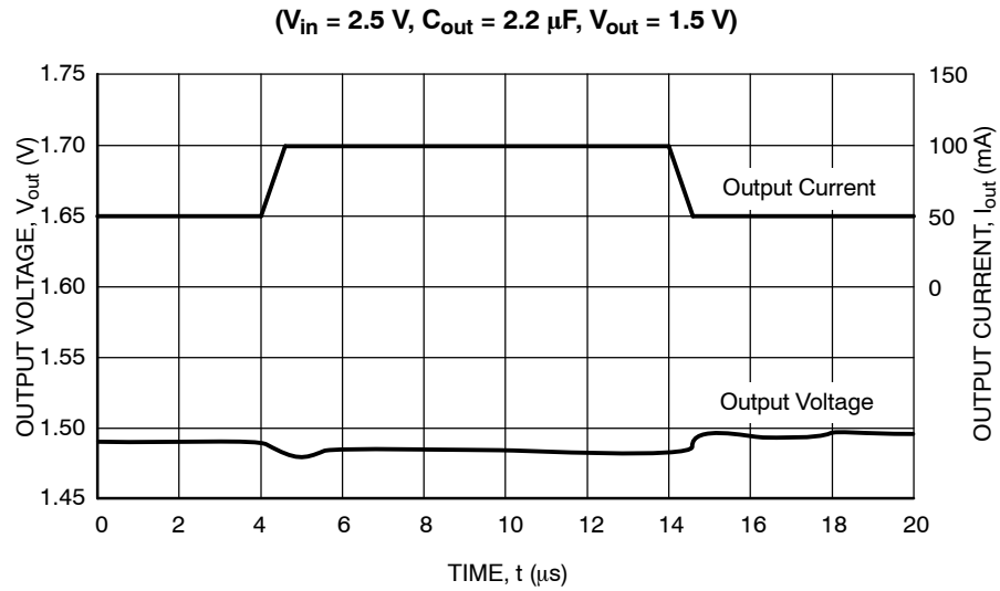
Figure 21. Load Transient Response ( t_r = t_f = 0.5\text{ }\mu\text{s} , C_{in} = 1.0\text{ }\mu\text{F} )
