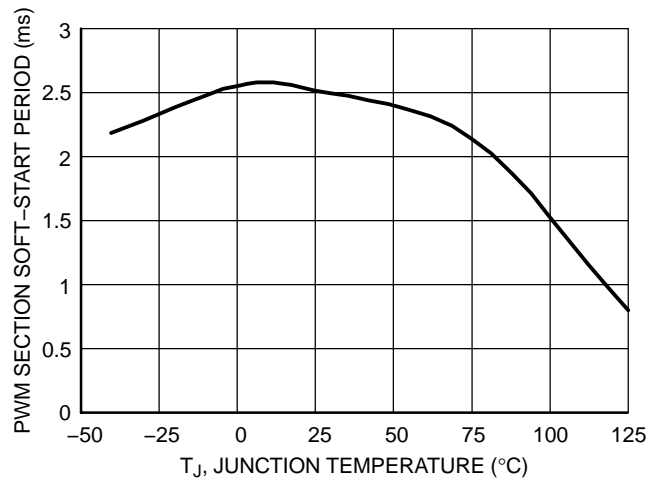
Figure 8. PWM Section Soft-Start/Soft-Skip Period vs. Temperature
