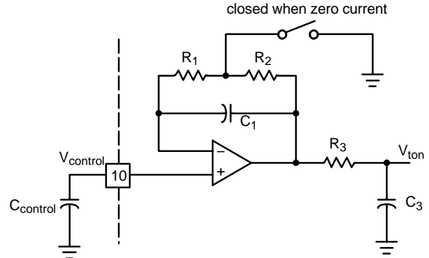
Figure 61. V_{control} Processing Circuit
