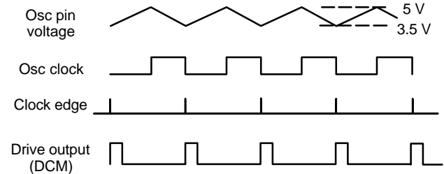
Figure 69. Oscillator Mode Timing Diagram in DCM
