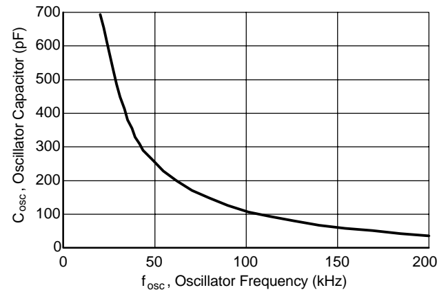
Figure 70. Osc Pin Frequency Setting
