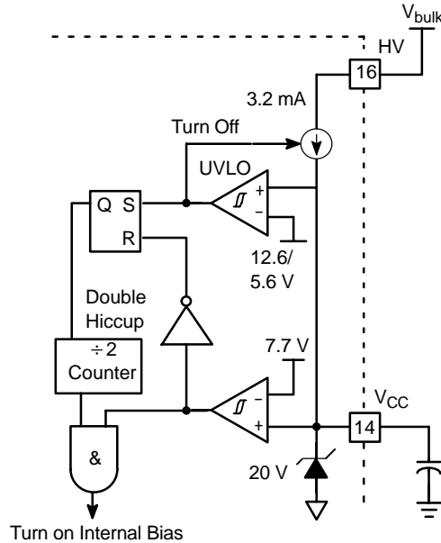
Figure 48. V_{CC2} Management
