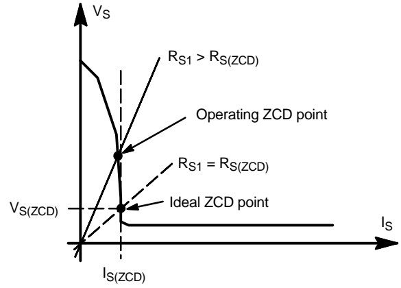
Figure 65. CS Pin Characteristic when I_L = 0
