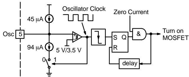
Figure 67. Oscillator / Synchronization Block in PFC Section
