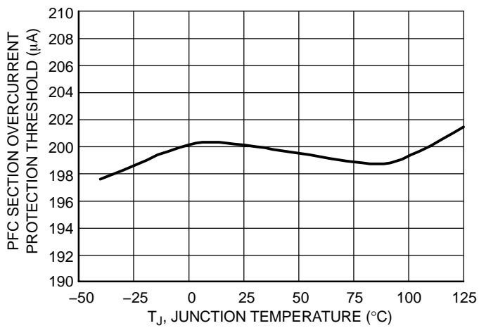
Figure 37. PFC Section Overcurrent Protection Threshold vs. Temperature
