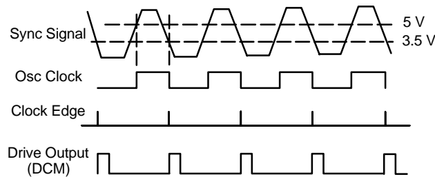
Figure 71. Synchronization Mode Timing Diagram in DCM
