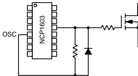
Figure 72. Synchronization Configuration
