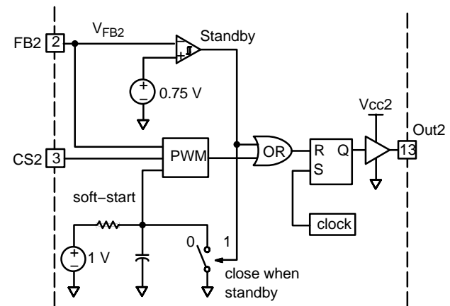
Figure 56. Block Diagram in Standby Operation
