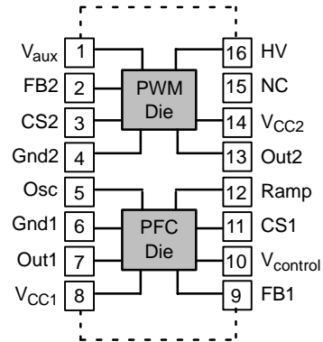
Figure 46. Internal Connection
