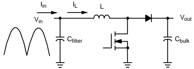
Figure 58. DCM/CRM PFC Boost Converter
