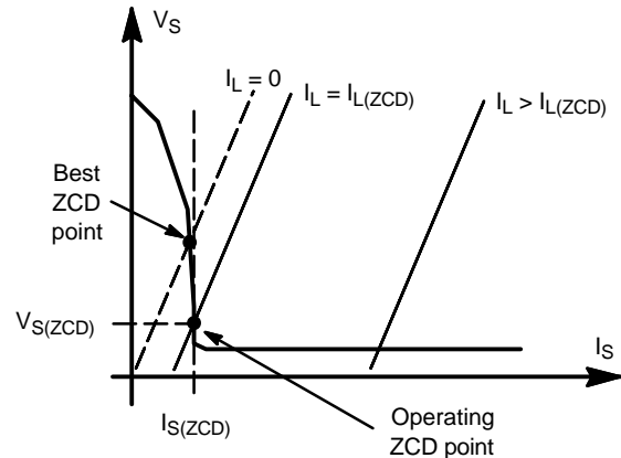
Figure 66. CS Pin Characteristic with Different Inductor Current
