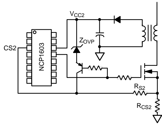
Figure 74. V_{CC} Latched OVP Application Circuit
