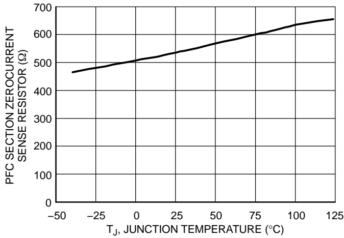
Figure 39. PFC Section Zerocurrent Sense Resistor vs. Temperature
