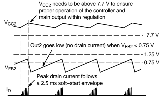
Figure 55. Timing Diagram in Standby Condition
