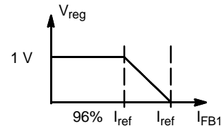
Figure 63. Regulation Block
