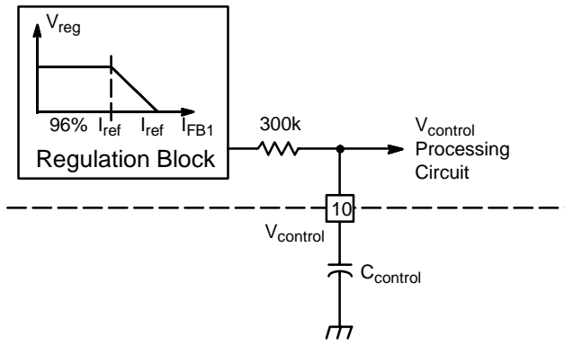
Figure 62. V_{\text{control}} Low-Pass Filtering
