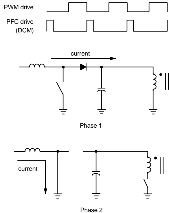
Figure 73. Synchronization Timing Diagram
