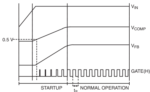
Figure 20. Idealized Waveforms
