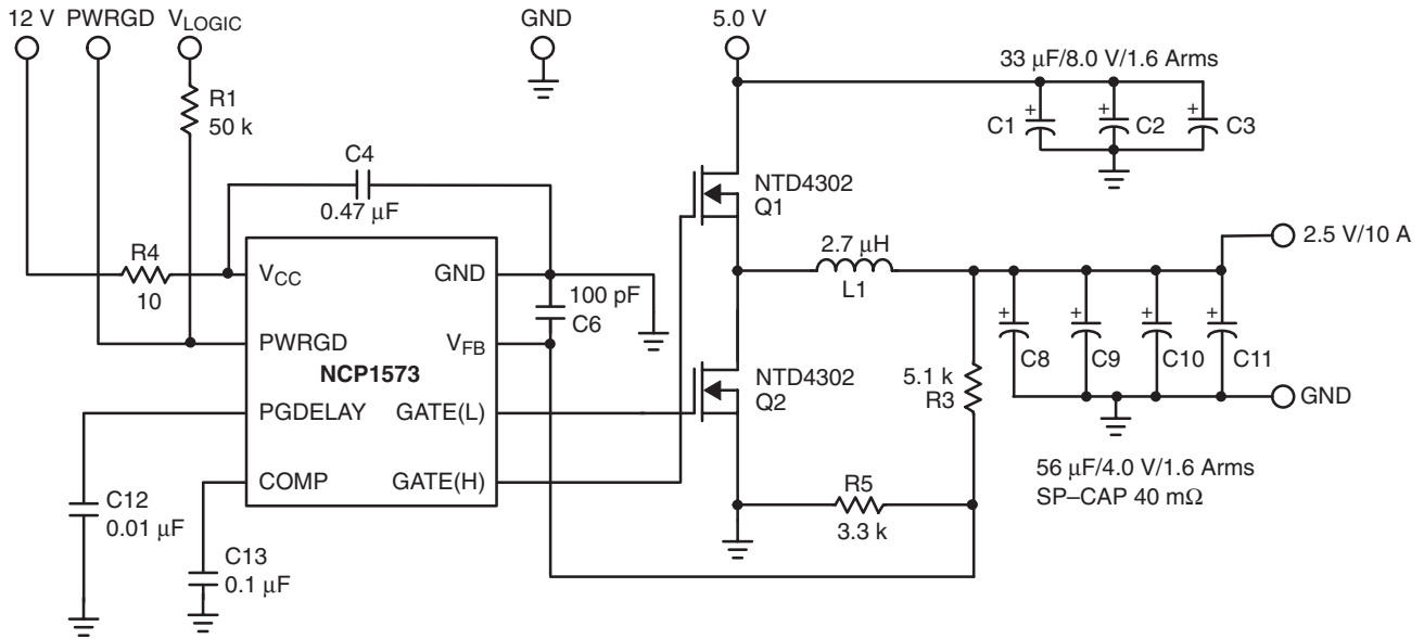
Figure 1. Applications Circuit
