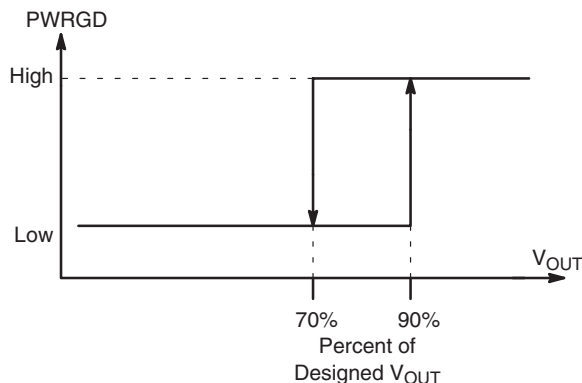
Figure 21. PWRGD Assertion
