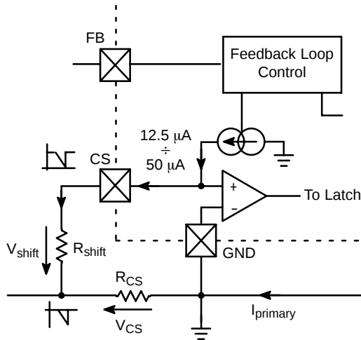
Figure 19. Primary Current Sensing
