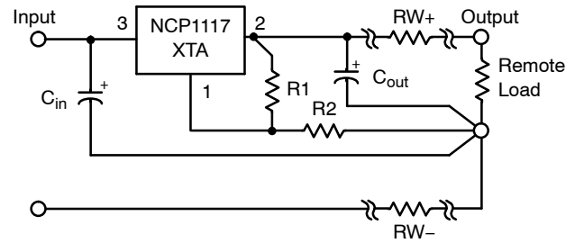
Figure 23. Load Sensing
