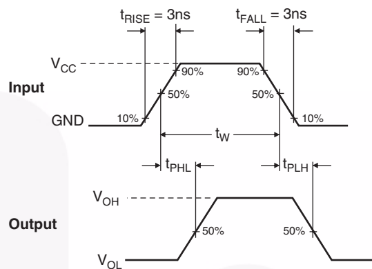
Figure 2. AC Waveforms
