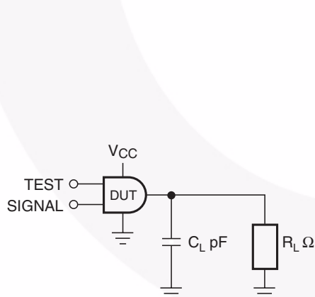
Figure 1. AC Test Circuit
