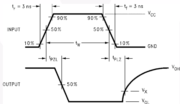
Figure 2. Waveform for Inverting and Non-Inverting Functions
