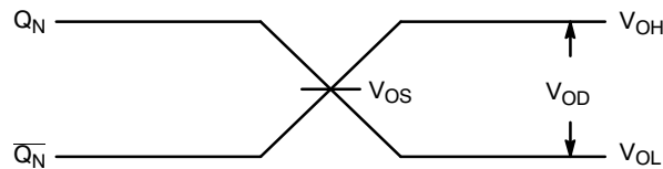
Figure 14. LVDS Output
