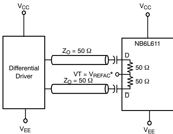
Figure 14. Capacitor-Coupled Differential Interface ( V_T Connected to V_{REFAC} )
