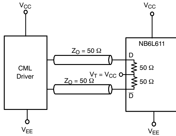
Figure 13. Standard 50 \Omega Load CML Interface
