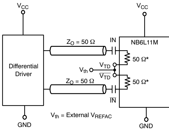
Figure 13. Capacitor-Coupled Differential Interface ( V_{TD}/\bar{V}_{TD} Connected to V_{REFAC} ; V_{REFAC} Bypassed to Ground with 0.1 \mu\text{F} Capacitor)
