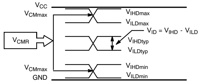
Figure 13. V_{CMR} Diagram
