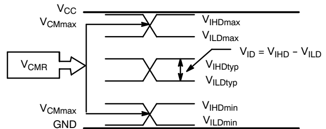
Figure 18. V_{CM} Diagram
