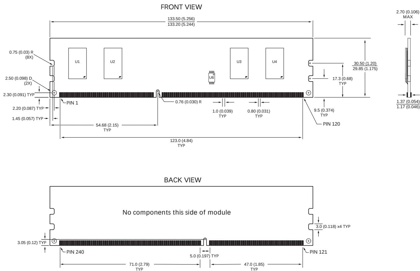
Figure 3: 240-Pin DDR3 UDIMM
