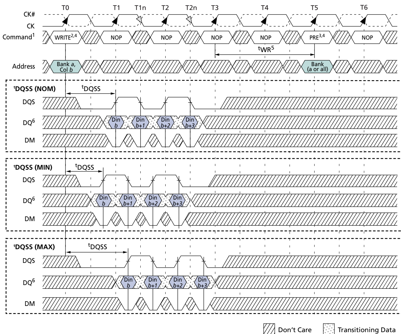
Figure 41: WRITE-to-PRECHARGE – Uninterrupting
