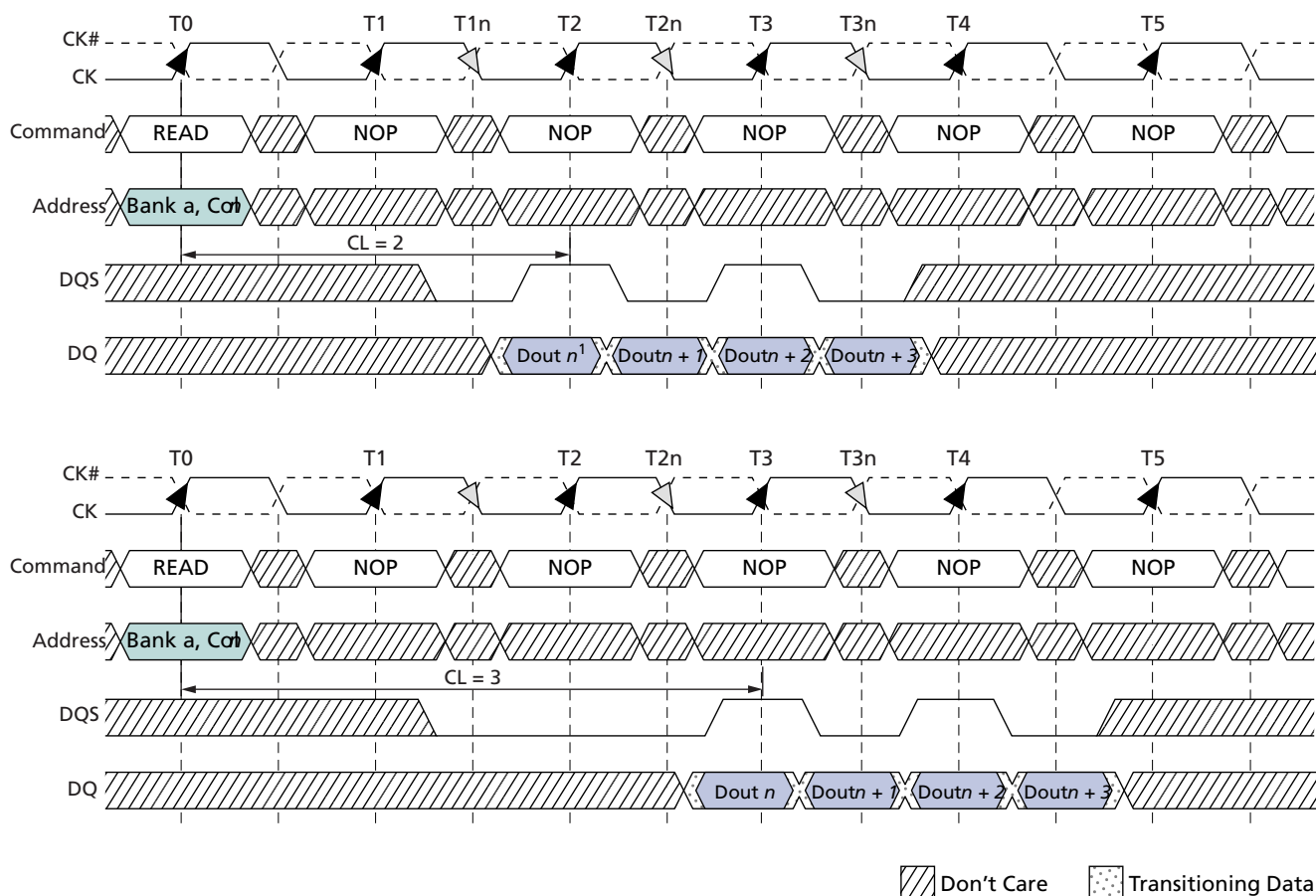
Figure 22: READ Burst
