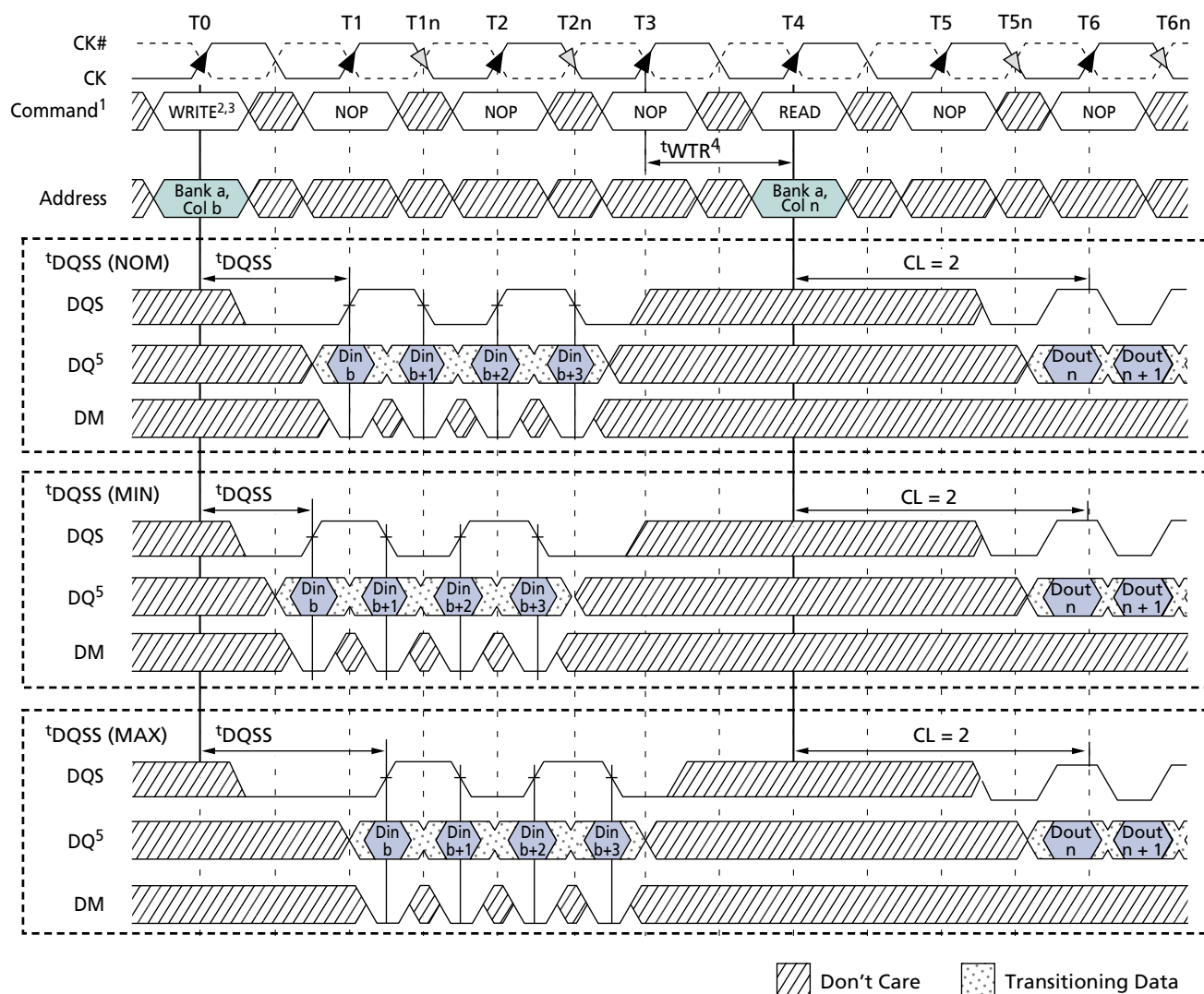
Figure 38: WRITE-to-READ – Uninterrupting
