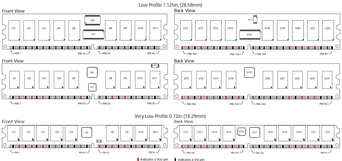
Figure 2: Pin Locations
