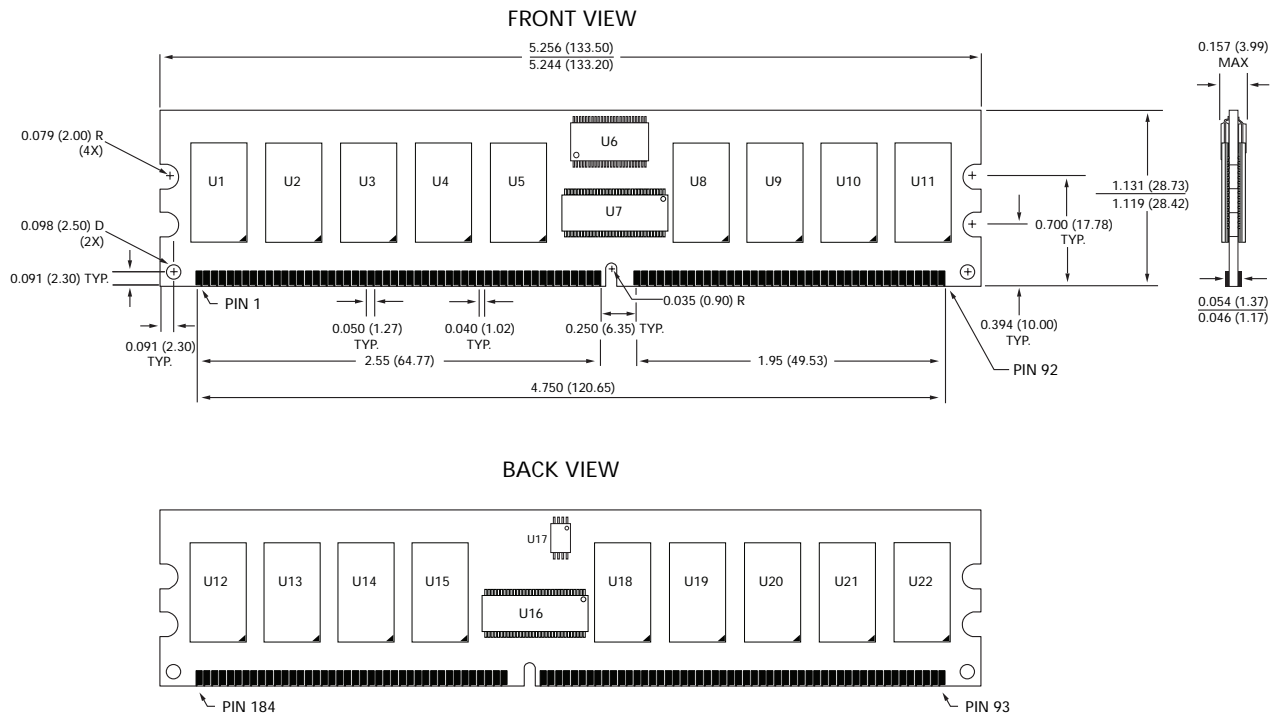
Figure 19: 184-Pin DIMM Dimensions – Alternate Low-Profile PCB
