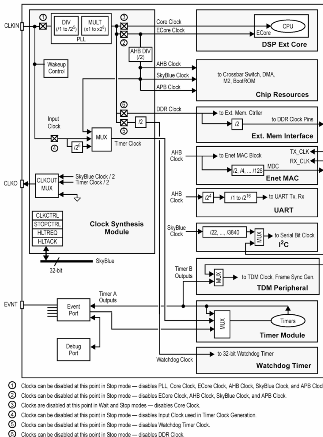
Figure 4-2. EVM Timing System
