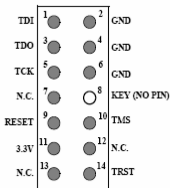
Figure 3-6. JTAG/OCE10 Connector, Front View
