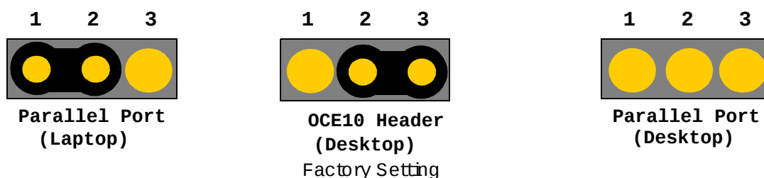
Figure 2-2. JP1- Host Terminal Connection
