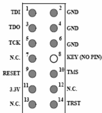
Figure 4-6. JTAG/OCE10 Port Connector
