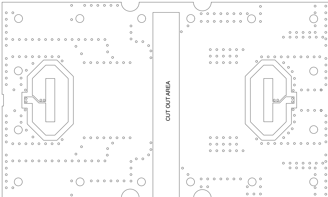
Figure 3a. MRF6VP3450HR6(HSR6) Test Circuit Component Layout — Bottom
