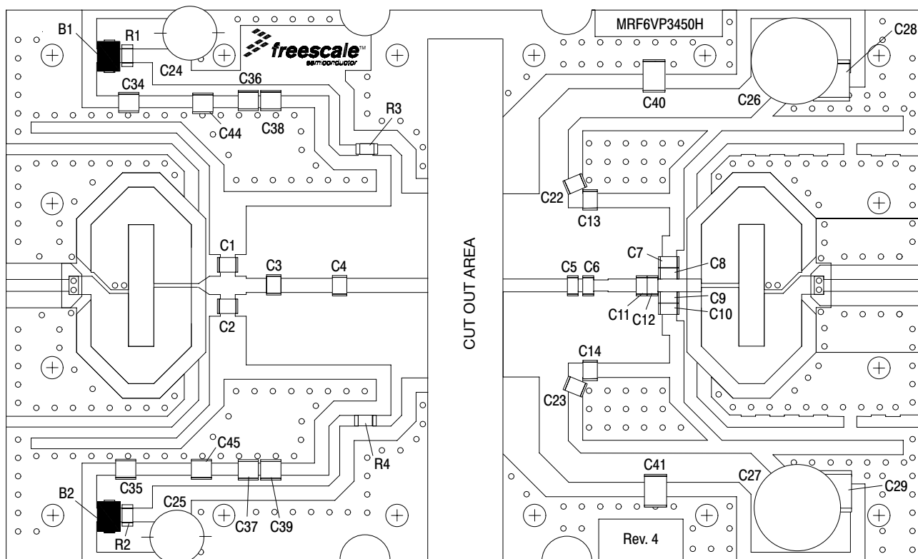
Figure 3. MRF6VP3450HR6(HSR6) Test Circuit Component Layout — Top
