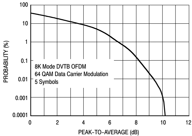
Figure 14. Single-Carrier DVB OFDM
