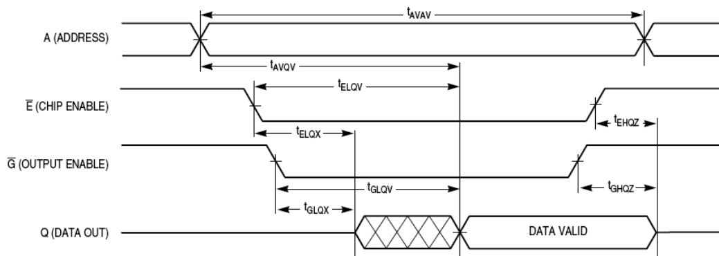
Figure 5. Read Cycle 1
