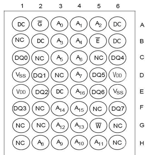
48-Pin FBGA
