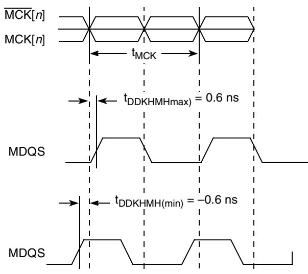
Figure 3. Timing Diagram for t_{DDKMH}
