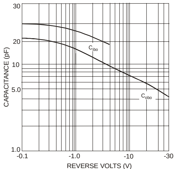
Fig. 3 Typical Capacitance
