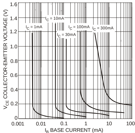
Fig. 4 Typical Collector Saturation Region
