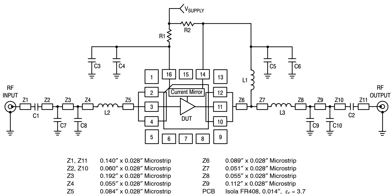
Figure 4. 50 Ohm Test Circuit Schematic
