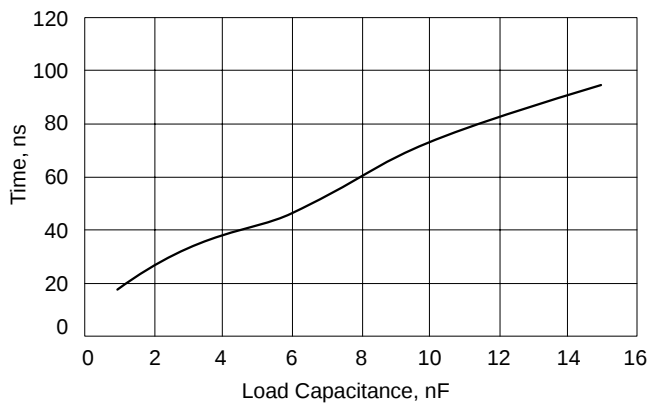
Figure 7. Gate(H) Fall-time vs. Load Capacitance measured from 4 V to 1 V with V_{CC} at 5 V.
