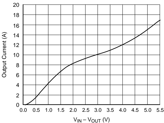
Figure 9. Short Circuit vs. V_{\text{IN}} - V_{\text{OUT}}
