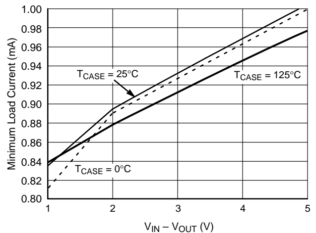
Figure 10. Minimum Load Current vs. V_{\text{IN}} - V_{\text{OUT}}
