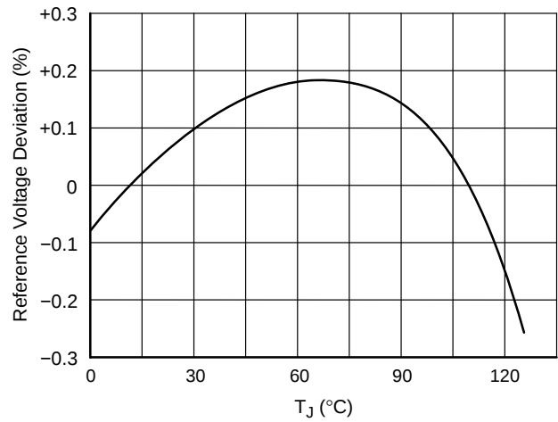
Figure 4. Output Voltage Deviation vs. Temperature
