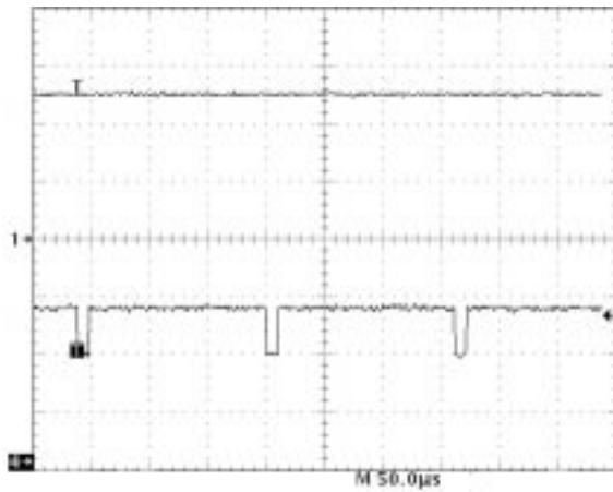
Figure 26. Power Good is Insensitive to Out of Regulation Conditions that are Present for a Duration Less Than the Built In Delay
