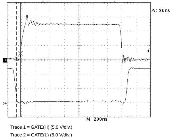
Figure 29. Normal Operation Showing the Guaranteed Non-Overlap Time Between the High and Low-Side MOSFET Gate Drives, I LOAD = 14 A
