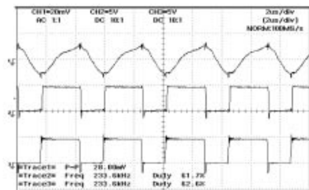
Figure 32. No Load Waveforms
