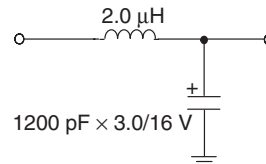
Figure 22. Input Filter
