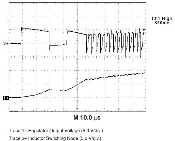
Figure 6. CS5160 Enable Startup Waveforms
