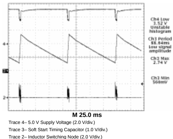
Figure 12. CS5158 Demonstration Board Hiccup Mode Short Circuit Protection. Gate Pulses are Delivered While the Soft Start Capacitor Charges, and Cease During Discharge
