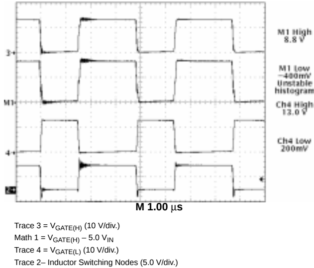
Figure 19. CS5158 Gate Drive Waveforms Depicting Rail to Rail Swing
