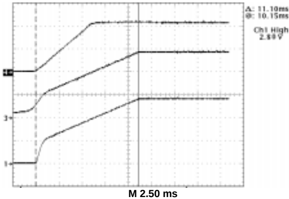
Figure 4. CS5158 Demonstration Board Startup in Response to Increasing 12 V and 5.0 V Input Voltages. Extended Off Time is Followed by Normal Off Time Operation when Output Voltage Achieves Regulation to the Error Amplifier Output.
