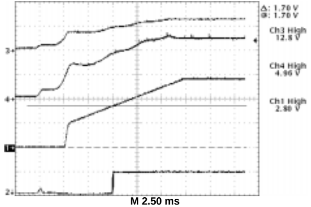
Figure 17. Implementing Power Good with the CS5157
