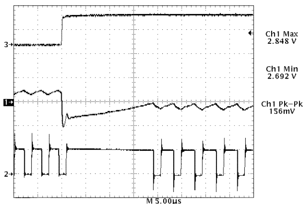
Figure 9. CS5156H Demonstration Board Response to a 0.5 to 13 A Load Pulse (Output Set for 2.8 V)
