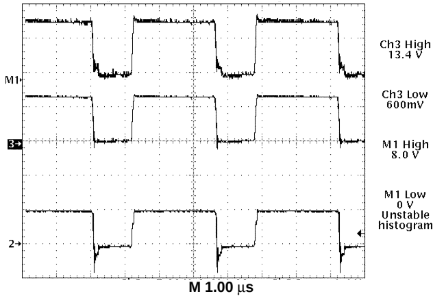
Figure 17. CS5156H Gate Drive Waveforms Depicting Rail to Rail Swing
