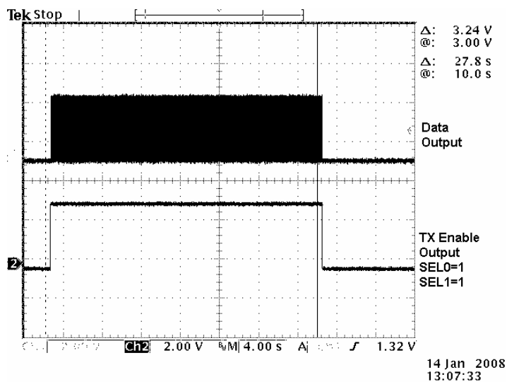
Figure 9. MICRF302 Time
