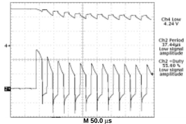
Figure 12. CS5155H Demonstration Board Hiccup Mode Short Circuit Protection. Gate Pulses are Delivered While the Soft Start Capacitor Charges, and Cease During Discharge
