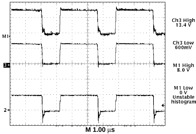
Figure 17. CS5151H Gate Drive Waveforms Depicting Rail to Rail Swing
