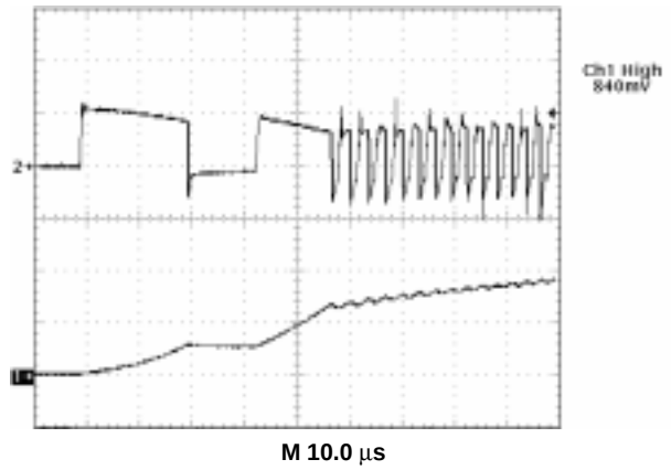
Figure 6. CS5151H Demonstration Board Enable Startup Waveforms
