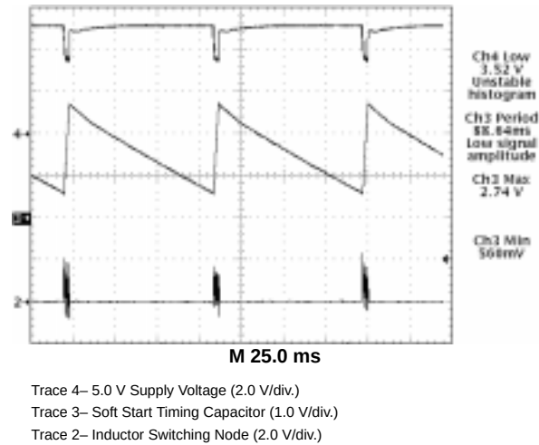
Figure 12. CS5151H Demonstration Board Hiccup Mode Short Circuit Protection. Gate Pulses are Delivered While the Soft Start Capacitor Charges, and Cease During Discharge
