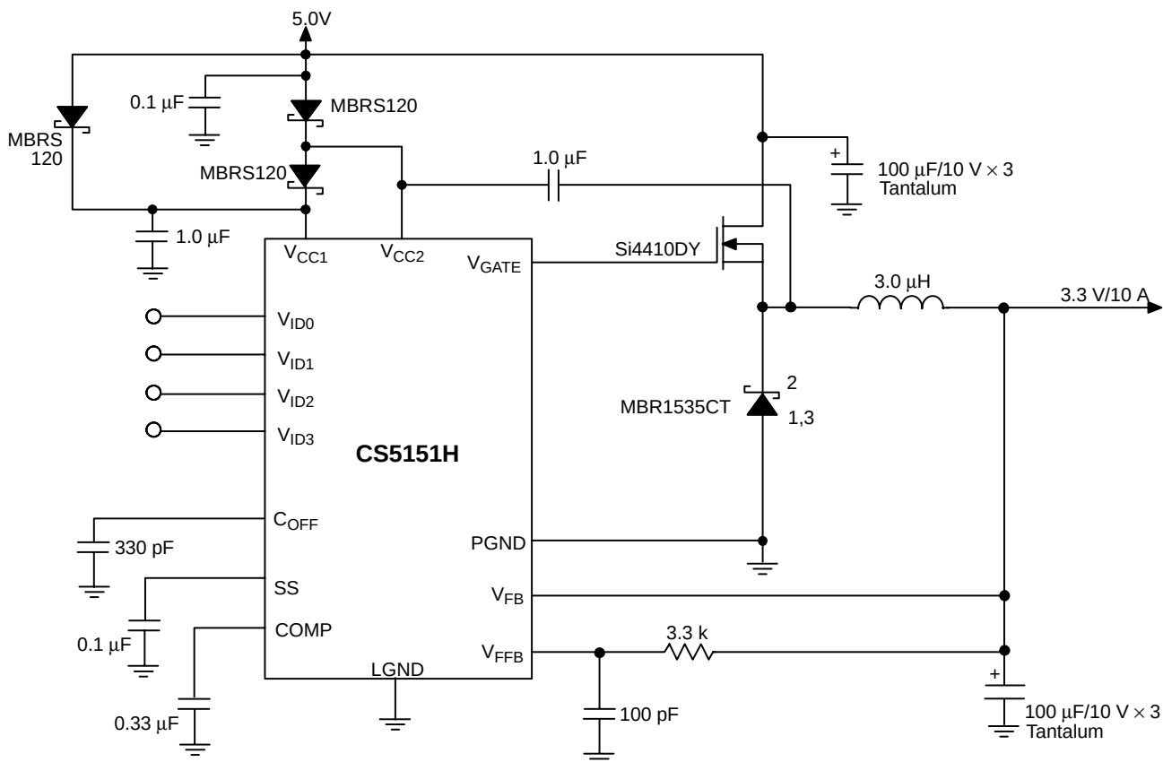
Figure 21. Additional Application Diagram, 5.0 V to 3.3 V/10 A Converter
