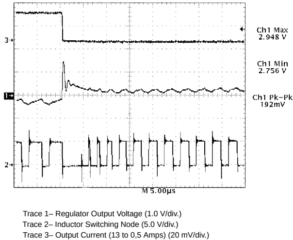
Figure 11. CS5151H Demonstration Board Response to 13 A Load Turn Off (Output Set for 2.8 V). V 2 Control Topology Immediately Connects Inductor to Ground, Providing 0% Duty Cycle. Regulation is Achieved in Less Than 10 μs
