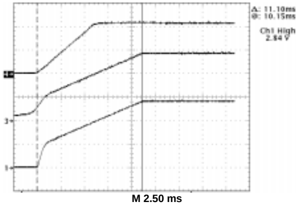
Figure 4. CS5151H Demonstration Board Startup in Response to Increasing 12 V and 5.0 V Input Voltages. Extended Off Time is Followed by Normal Off Time Operation when Output Voltage Achieves Regulation to the Error Amplifier Output.
