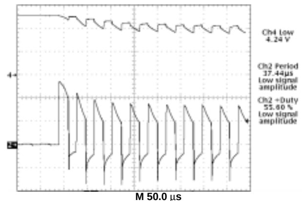
Figure 12. CS5151 Demonstration Board Hiccup Mode Short Circuit Protection. Gate Pulses are Delivered While the Soft Start Capacitor Charges, and Cease During Discharge
