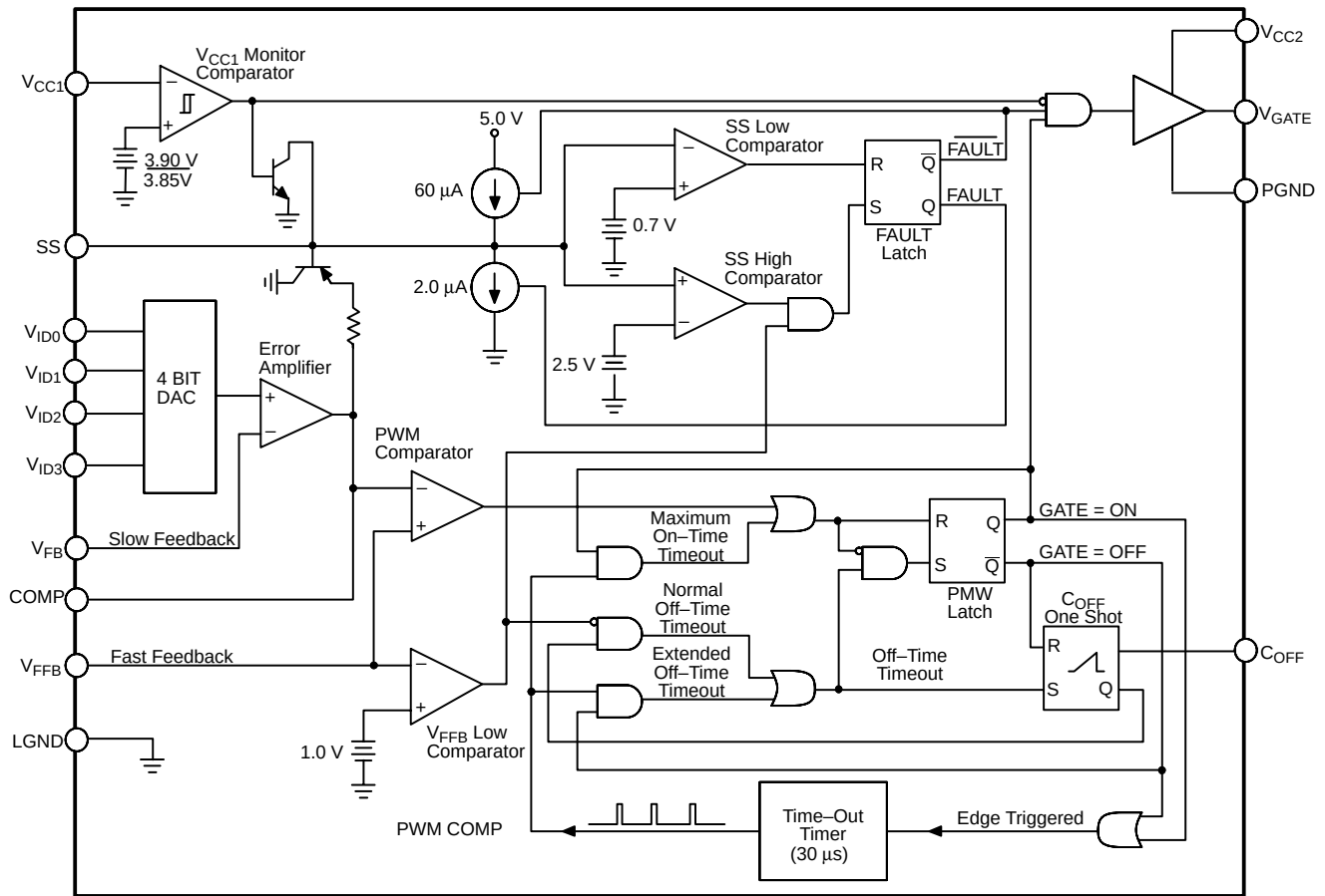
Figure 2. Block Diagram
