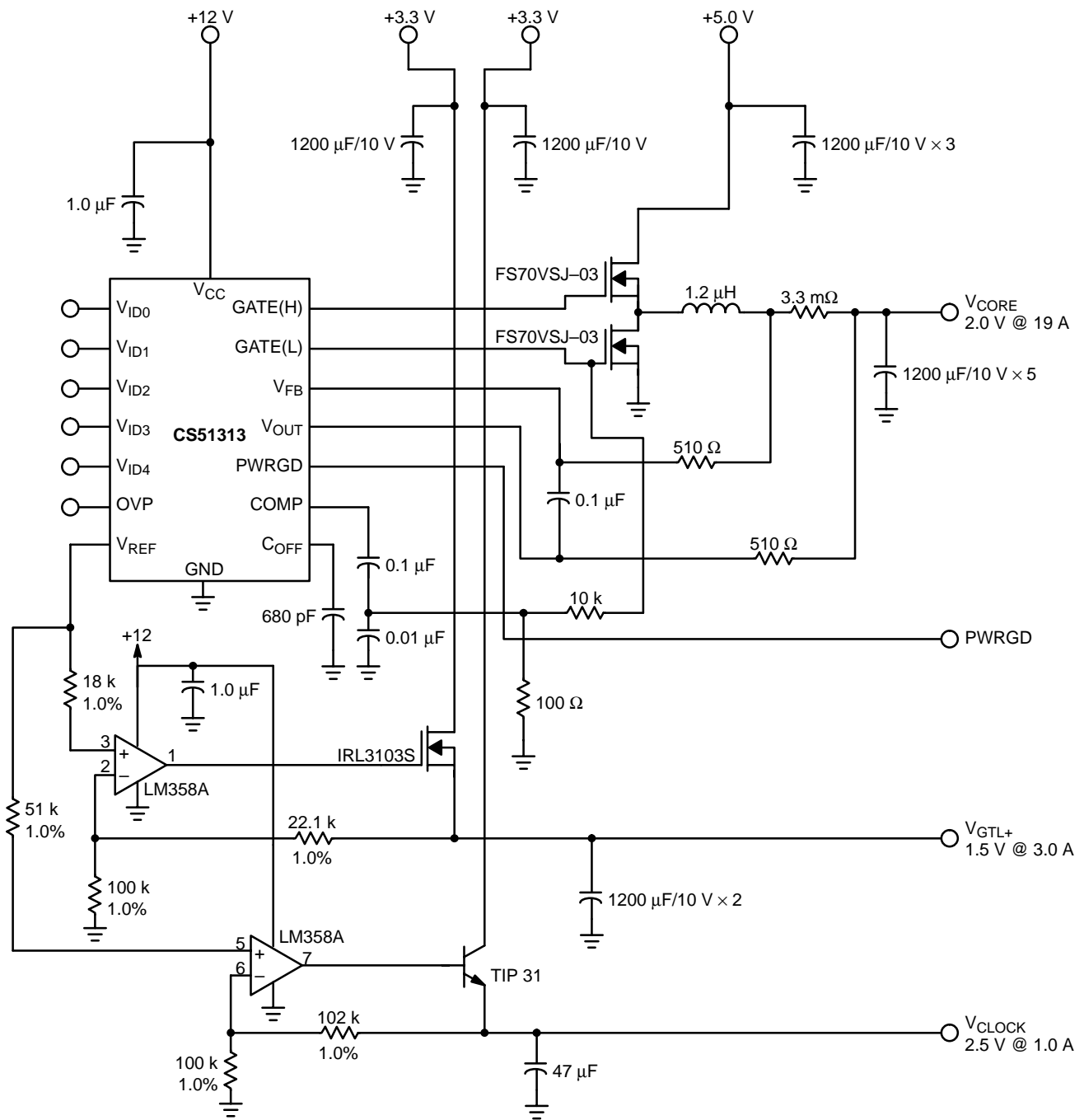
Figure 1. Application Diagram
