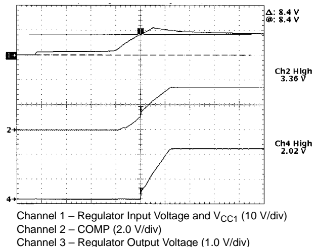
Figure 10. Normal Startup (5.0 ms/div)
