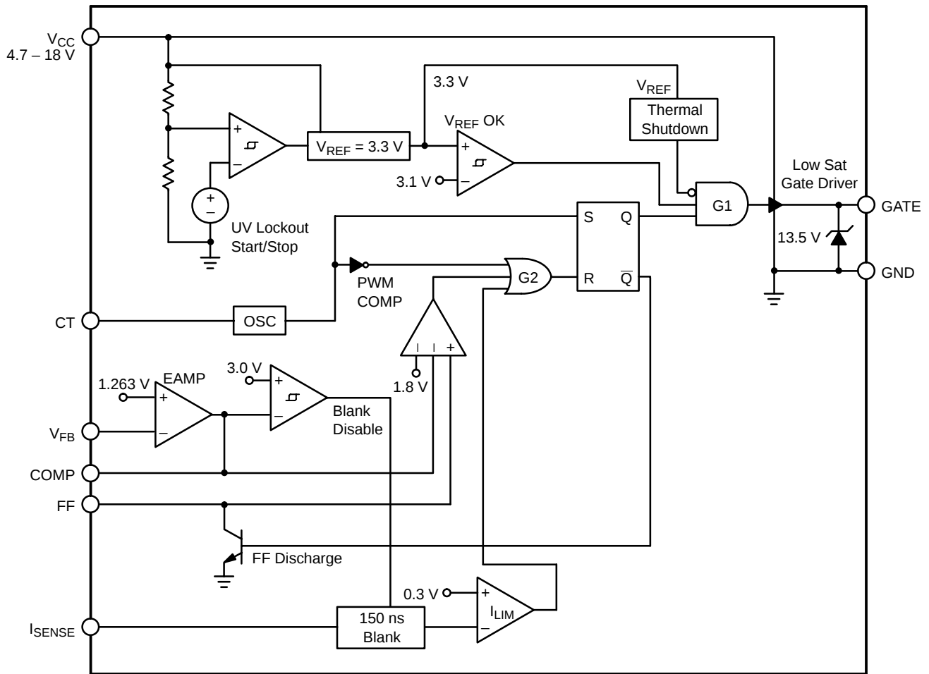
Figure 2. Block Diagram
