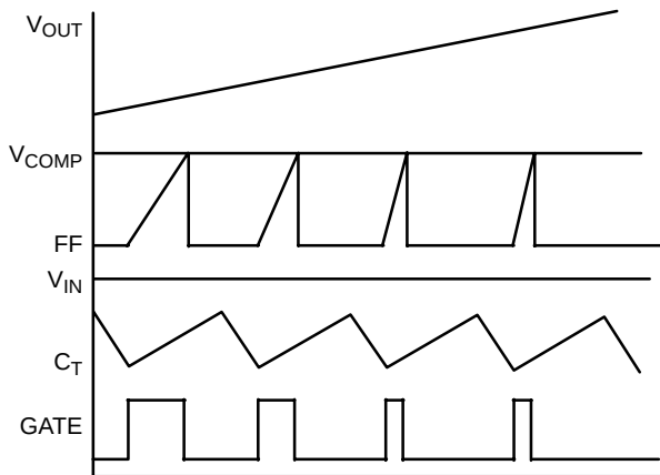
Figure 5. Pulse Width Modulated By Input Voltage With Constant Output Voltage
